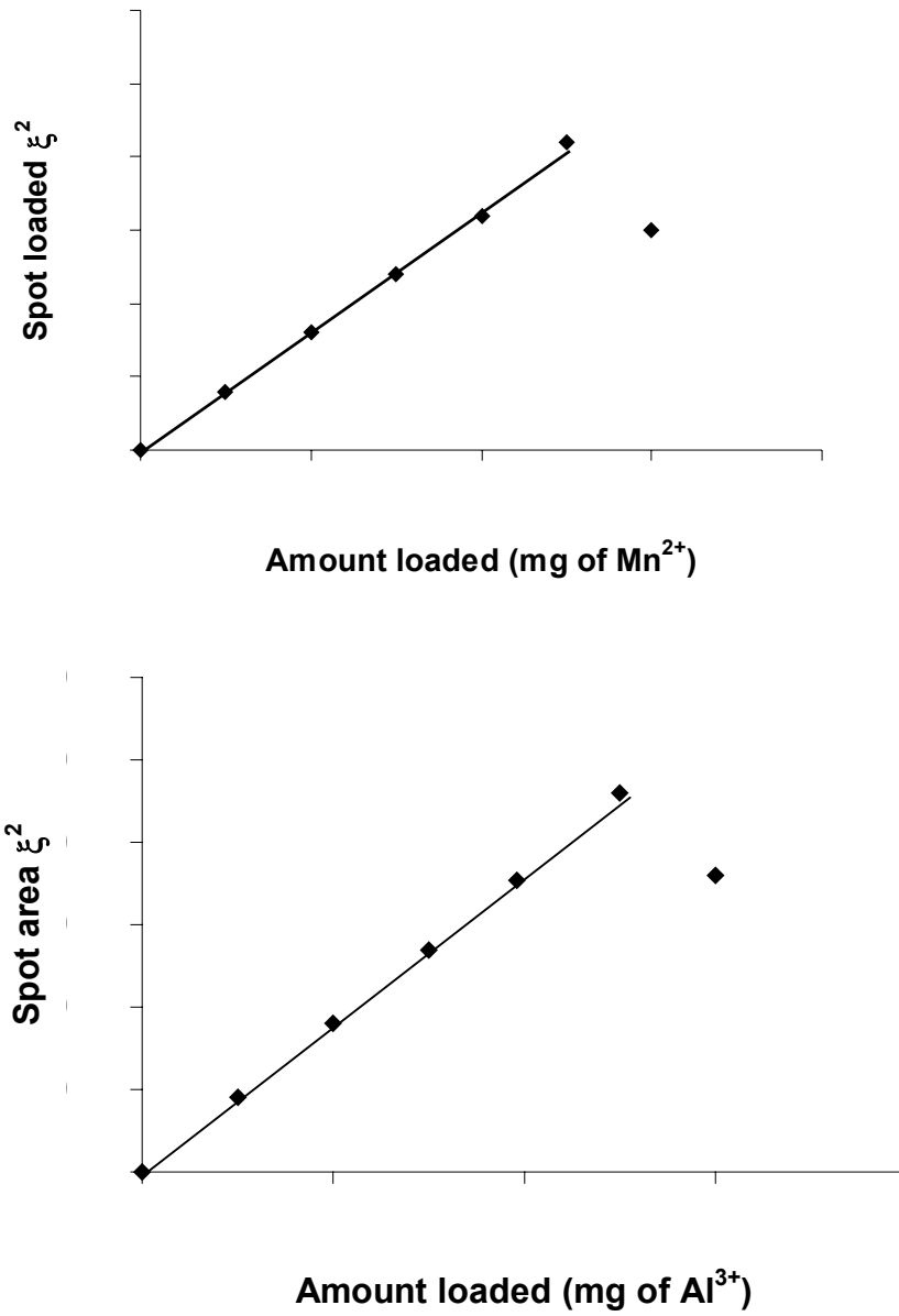
Fig. 2 Calibration plots for semiquantitative determination of (a) Mn 2+ and (b) Al 3+
